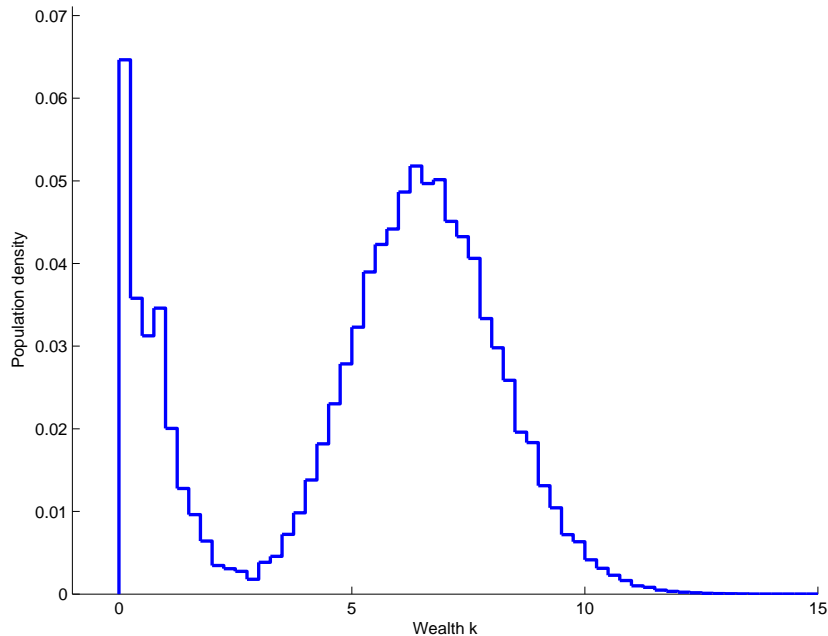
Figure 4: Steady state wealth distribution for \Theta = \{\theta_0, 0.4\}
