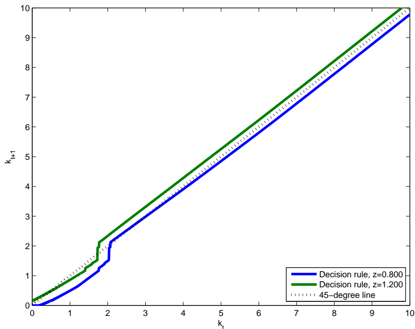
Figure 5: Decision rule in steady state (only k < 10 shown) ( \Theta = \Theta_0, \mu = 0.5, w = 1.492 )
