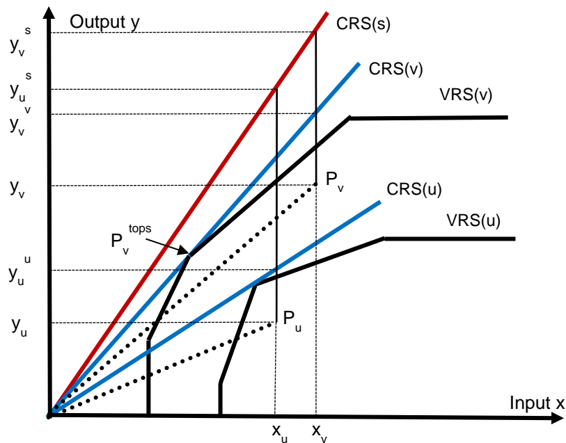
Figure 2. The Malmquist productivity change index. Productivity change for a unit from period u to period v measured relative to the benchmark CRS(s) envelopment with maximal productivity of the pooled dataset
