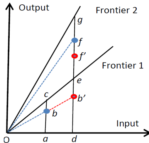
Figure 4. The decomposition of the Malmquist index
