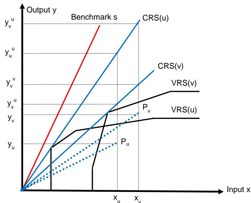
Figure 6. Contemporaneous cones and VRS technologies
