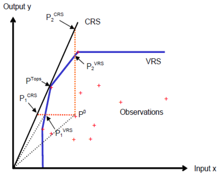
Figure 1. The Farrell efficiency measures applied to a piecewise linear VRS frontier
