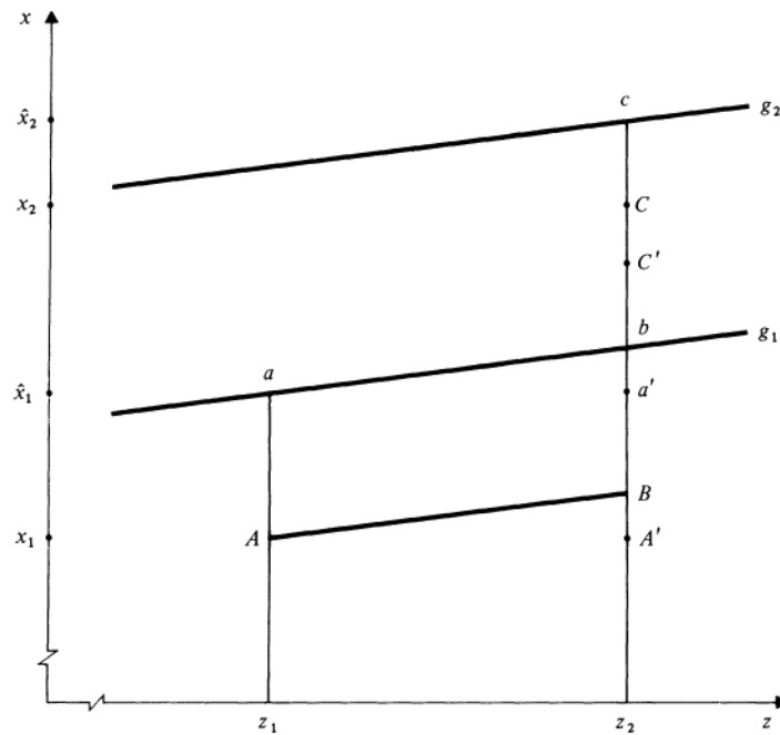
Fig. 1. Alternative interpretations of productivity change.
